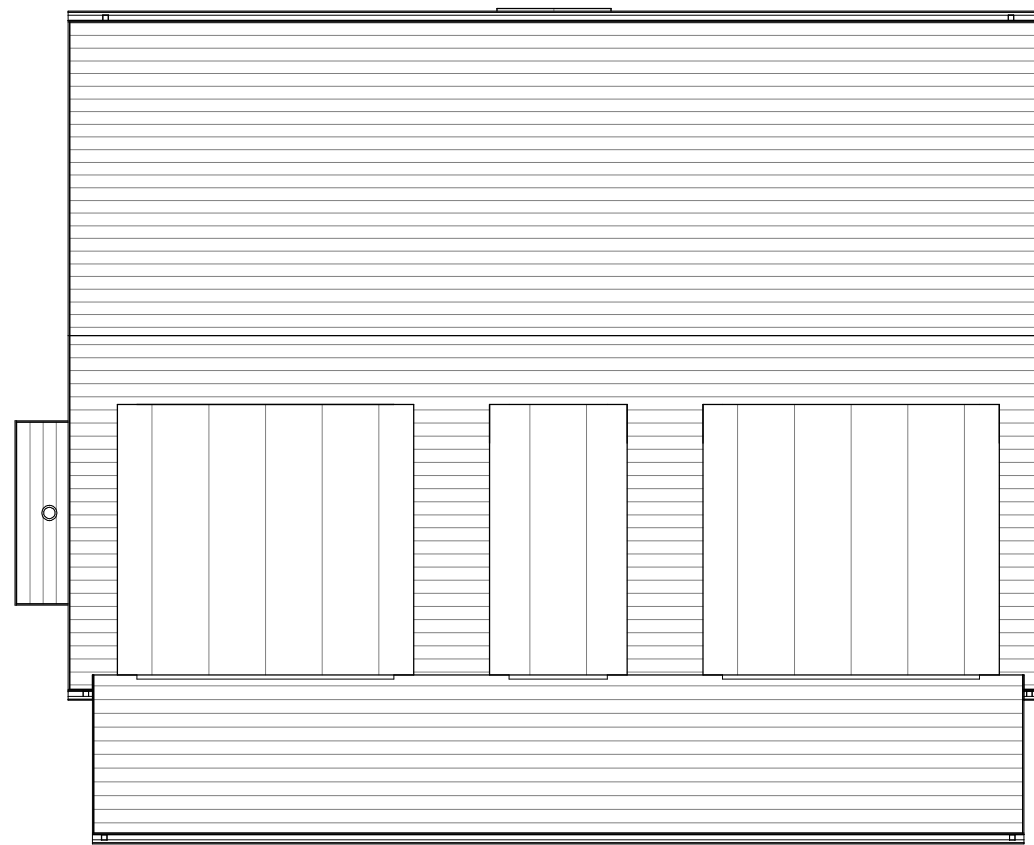
ROOF PLAN
