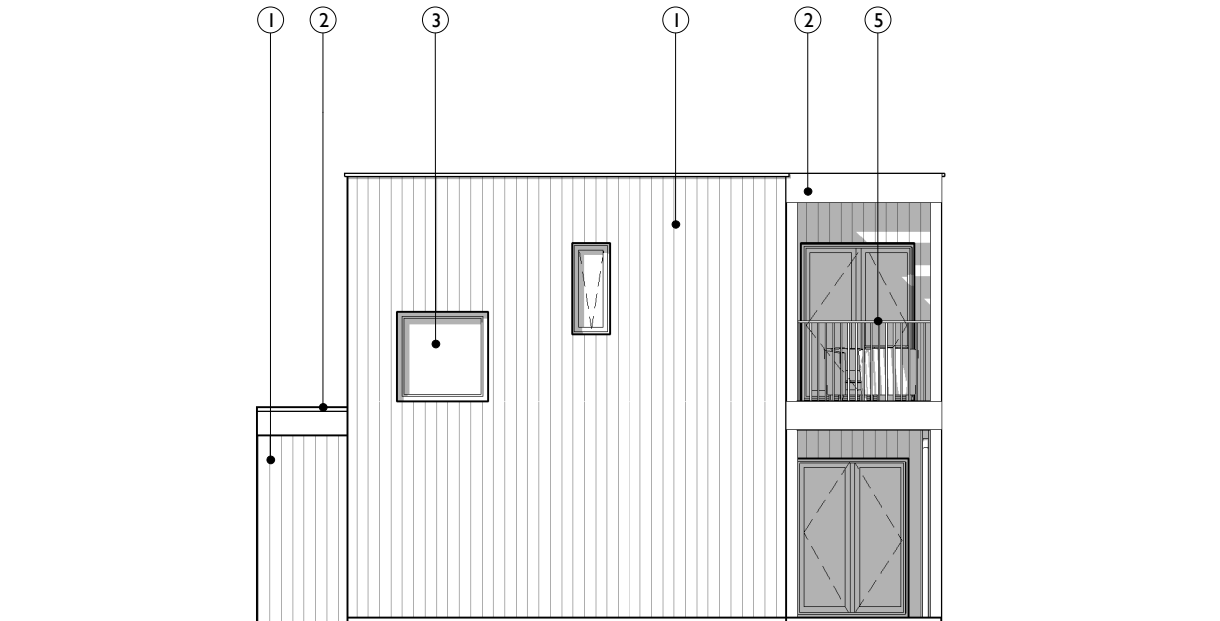
SIDE ELEVATION
