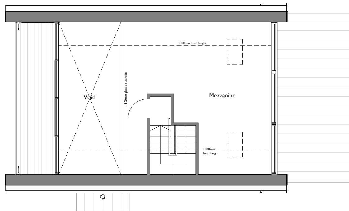
MEZZANINE FLOOR PLAN
